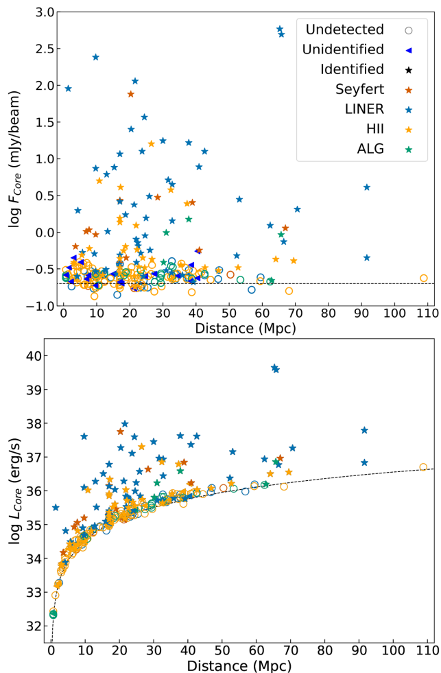
Figure 5. Radio core flux density ( F_{\text{core}} in \text{mJy beam}^{-1} , upper panel) and its luminosity ( L_{\text{core}} , integrated over the e -MERLIN L band, 1.244–1.756 GHz, in \text{erg s}^{-1} , lower panel) as a function of distance (Mpc) for the full sample. The dashed lines represents the 3\sigma flux density limit of this survey ( 0.25 \text{ mJy beam}^{-1} ) and the corresponding luminosity, respectively, in the upper and lower panels. The symbols in the legend indicate the status of their detection (open circles for undetected and filled stars for detected) and their optical class (red Seyferts, light blue LINERs, yellow H II galaxies, and green ALGs). For the unidentified (blue left-pointing triangles) and undetected radio sources, the values on the y -axis should be understood as upper limits. The typical error bar on flux densities and luminosities is 20 per cent of the values. To convert the radio luminosities from \text{erg s}^{-1} to \text{W Hz}^{-1} at 1.5 GHz, an amount +16.18 should be subtracted from the logarithm of the luminosities presented in the graph.
