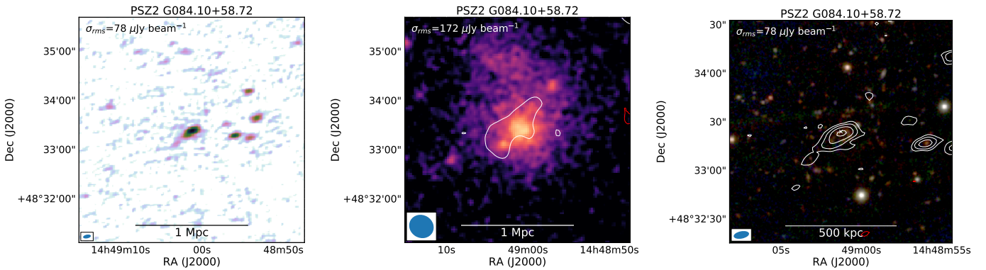
Fig. A.1. PSZ2 G084.10+58.72. Left : robust -0.5 radio image. Middle : XMM-Newton X-ray image with 15'' tapered radio contours (compact sources were subtracted). Right : optical image with robust -0.5 image radio contours. For more details, see the caption of Fig. 5.
