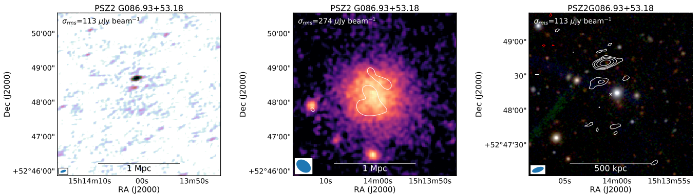
Fig. A.2. PSZ2 G086.93+53.18. Left : robust -0.5 radio image. Middle : XMM-Newton X-ray image with 15'' tapered radio contours (compact sources were subtracted). Right : optical image with robust -0.5 image radio contours. For more details, see the caption of Fig. 5.
