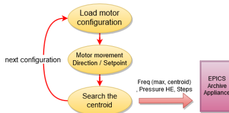
Figure 14: Sequence for the automatic cavity tuning measurement.
