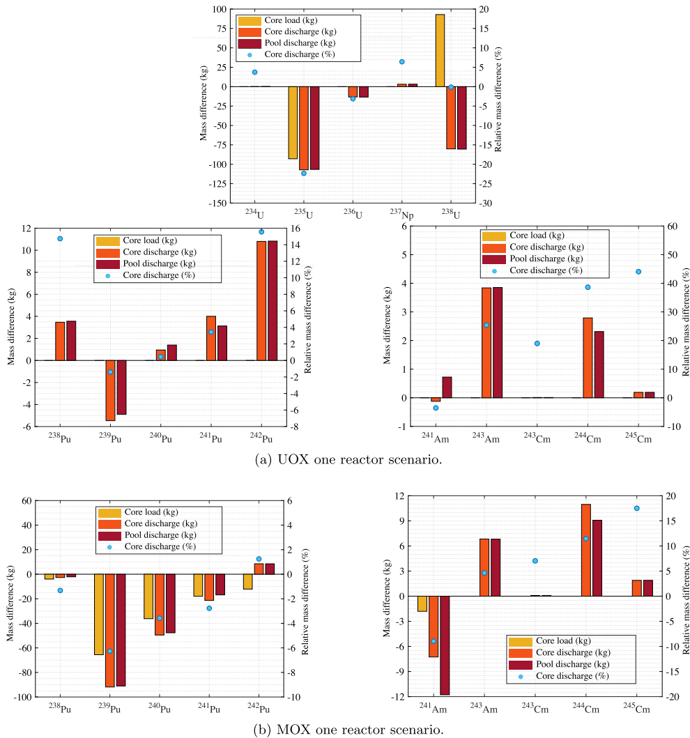
Fig. 11. Differences in isotopic inventories between CLASS-MLP and CLASS-DONJON5.
