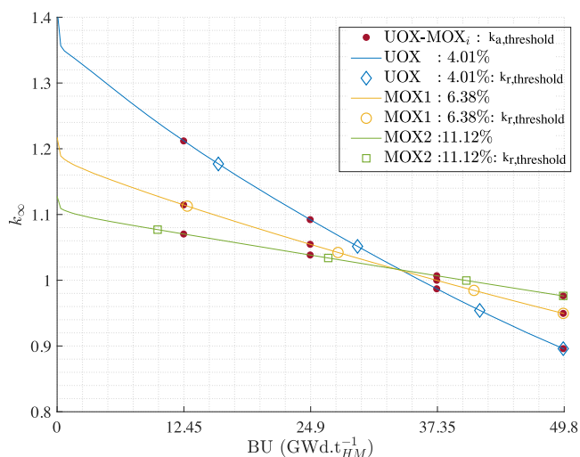
Fig. 9. Assembly reactivity evolution and reactivity at each refueling time evaluated with chained DONJON5-DRAGON5 calculations.
