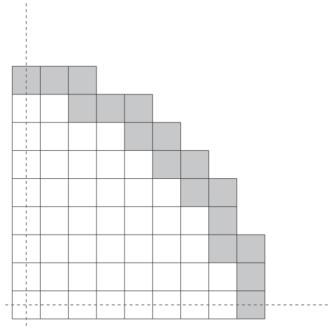
Fig. 4. Simulated quarter core layout (2D plane). Fuel assemblies (white) and reflector elements (gray) are displayed.
