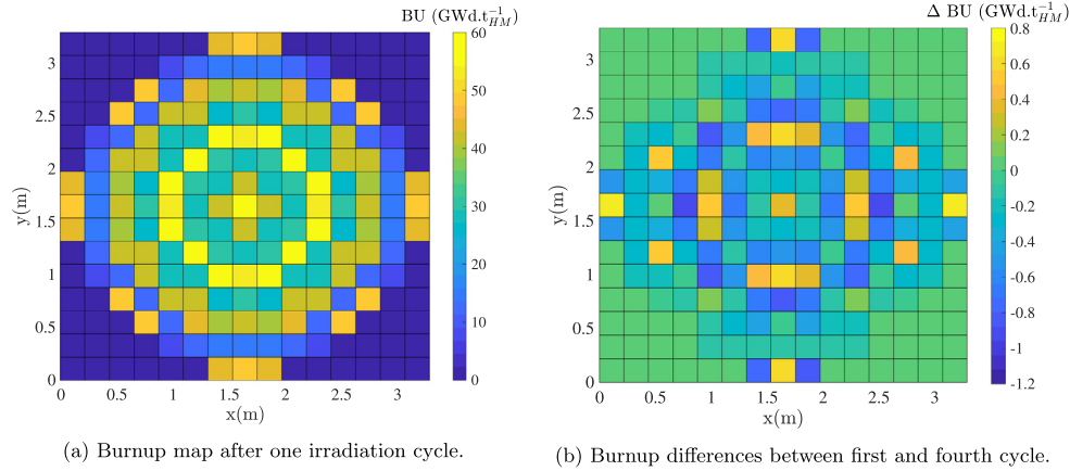
Fig. 7. MOX burnup predictions.
