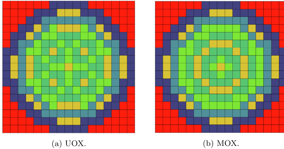
Fig. 5. Core loading patterns for UOX (a) and MOX (b) fuels. Red stands for void regions, dark blue for radial reflector material, light blue for new assemblies, and dark green, light green and yellow respectively for assemblies burned for one, two and three cycles.
