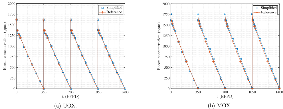
Fig. 8. In-core boron concentration for UOX (a) and MOX (b) fuels.
