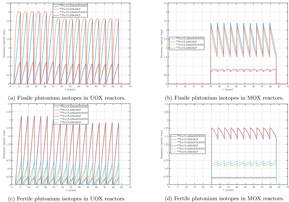
Fig. 14. In-core fertile and fissile plutonium for scenario OneBU.
