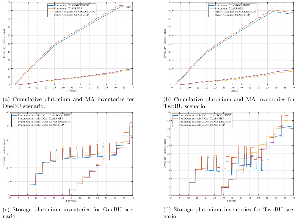
Fig. 13. Cumulative plutonium and minor actinides (MA) inventories from the fuel cycle and plutonium inventories in storage facilities for OneBU and TwoBU scenarios.
