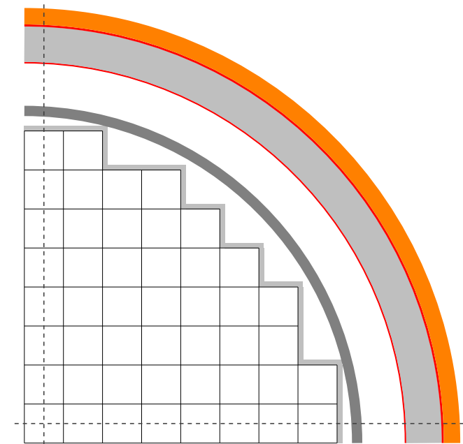
Fig. 3. Real quarter core layout (2D plane). Fuel assemblies (white), steel baffle (light gray), barrel (dark gray), steel vessel (gray) and thermal insulator (red and orange) are displayed.
