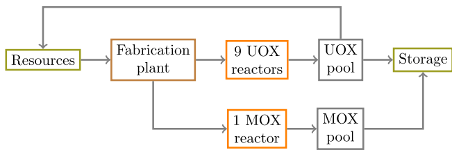
Fig. 12. Complex CLASS scenario with UOX-MOX fueled reactors interacting.
