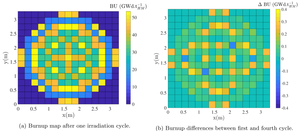
Fig. 6. UOX burnup predictions.
