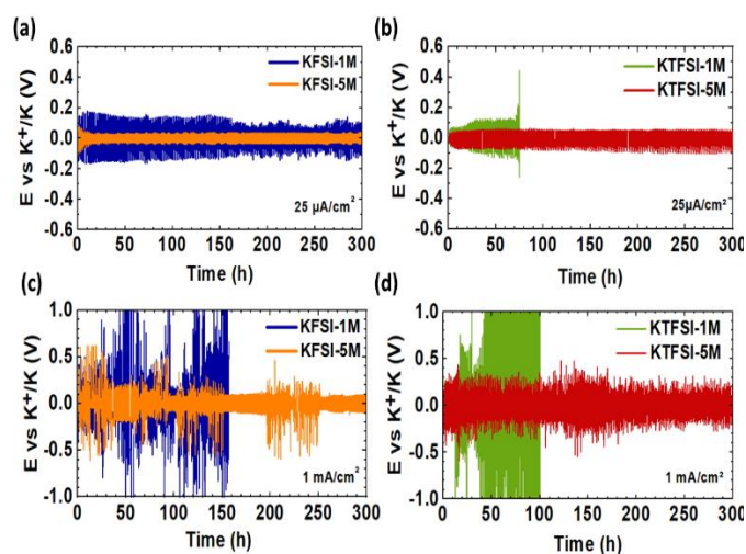
Figure 2. K-metal plating/stripping curves of K|K symmetric cells with KFSI-1M and KFSI-5M and KTFSI-1M and KTFSI-5M at a current density of 25 \mu\text{A/cm}^2 (a,b) and 1 \text{ mA/cm}^2 (c,d)
