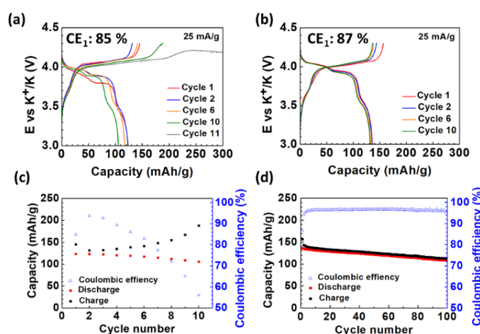
Figure 3. Galvanostatic profiles and long-term cycling evolution of PBA with KFSI-5M (a,c) and KTFSI-5M (b,d) recorded at 25 \text{ mA/g} between 3.0 and 4.3 V
