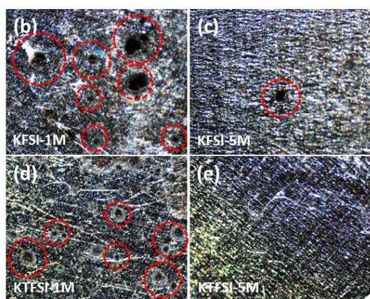
Figure 1. Linear sweep voltammetry of K-metal vs Al with the four electrolytes (a). Optical microscopy images (40X) of the Al current collector after the LSV of KFSI-1M (b), KFSI-5M (c), KTFSI-1M (d) and KTFSI-5M (e)
