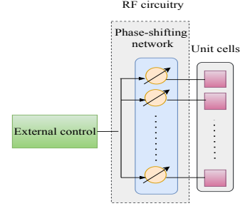
Fig. 3: Main RF circuitry of RISs.
