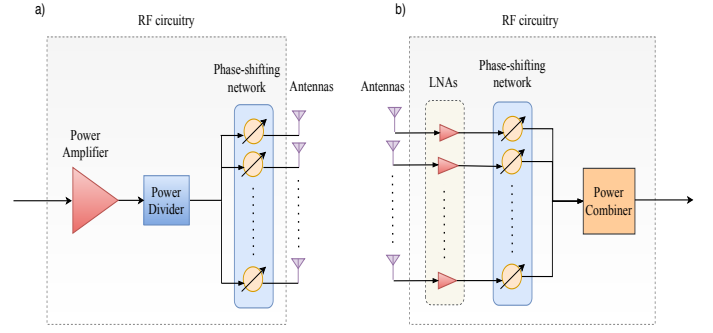
Fig. 2: Main RF circuitry used for a) transmission and b) reception in RRHs and relays.
