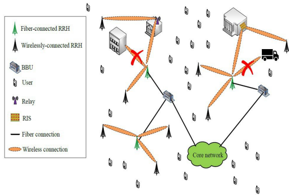
Fig. 1: Network layout.
