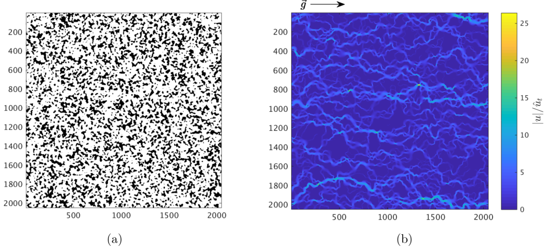
FIG. 2. (a) A typical reconstructed 2D porous domain used in this study. The black and white colors denote solid (impermeable to flow) and void (permeable) space, respectively. (b) Scaled velocity magnitude, |u|/\hat{u}_t , during creeping single-phase flow within the domain. Lighter colors correspond to higher velocities, while darker blue colors correspond to solid sites or flow stagnation regions. The calculated intrinsic permeability of the domain is k = 9.9\delta x^2 . Reported lengths are in lattice space units [\delta x] .
