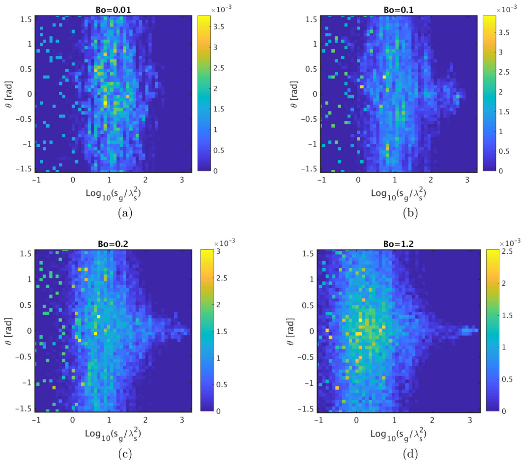
FIG. 10. Probability density maps of ganglia flow direction with respect to the applied body force, \theta , and size, s_g/\lambda_s^2 , over two orders of magnitude of Bo for S_{nw} = 0.4 . The scattered points in the left side of these maps should be attributed to very small stranded ganglia with sizes determined by the specific structural properties of our reconstructed domains. These constitute (at least partly) the reported residual saturation, S_{nw,r} .
