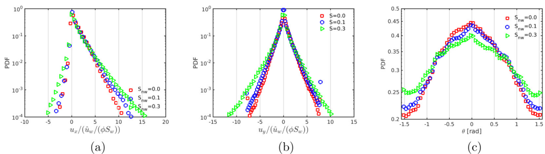
FIG. 12. Probability density functions (PDFs) of the rescaled (a) longitudinal, u_x , and (b) transverse velocity, u_y , components, and (c) orientation, \theta = \tan^{-1}(u_y/u_x) , of the w-phase velocity vector \vec{u}_w for various values of the nw-phase saturation in the limit where all ganglia are immobile (i.e., \text{Bo} \leq \text{Bo}_c ).
