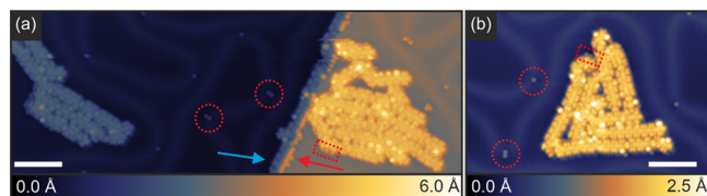
Figure 4. (a, b) Filled state STM images of chlorinated 5-AGNROHs after postsynthesis surface cleaning using 2.5 h molecular H 2 treatment at 180 °C. The red dashed circles, red arrow, and red dashed rectangle indicate residual bromine contamination; the blue arrow points to the molecules immobilized at a terrace step. Scanning parameters: –1 V, 100 pA; scale bar: 5 nm.
