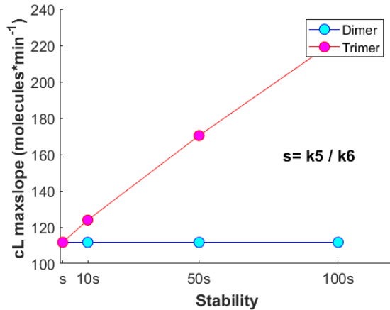
Figure 4. Increase in stability” of the trimeric complexes translate into higher cL maxslope values. The stability values in the trimeric complex are represented by means of “s” which refers to the ratio k5 / k6 .
