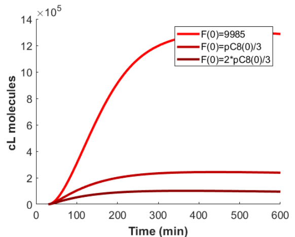
Figure 3. F inhibitory effect shows evidence of an irreversible-like reaction: A) Increasing the initial concentration F(0) from 9985 (fitted median_cell value) to 2p(0)/3 molecules ( \sim 140000 ) causes important variation on the maxslope of the simulated cL trajectory for decreasing F dissociation rates [k8, k10, k14] . B) Simulated cL trajectories for [k8, k10, k14]/100 and increasing F(0) levels. The maxslope of the trajectories decreases while gradually increasing F(0) .
