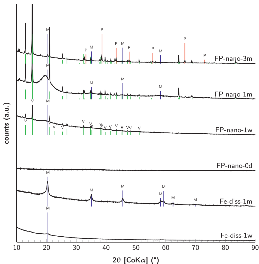
FIGURE 2 | X-ray diffractograms of solid phases in cultures after 1 week, 1 month, and 3 months as well as of initial nanoparticulate Fe III -phosphate. Characteristic peaks of reference minerals are indexed for mackinawite (blue), vivianite (green), and pyrite (red).
