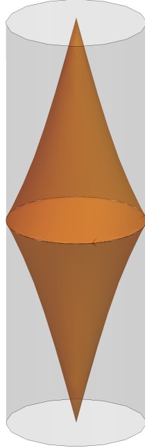
FIGURE 7. The invisible domain of the boundary of a spacelike plane in the Poincaré model for \widetilde{\text{AdS}}^{2,1} .
