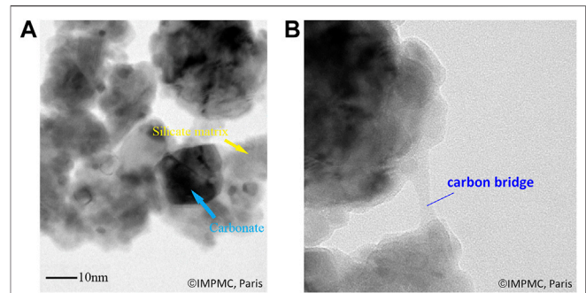
FIGURE 8 | TEM micrographs of carbonated slag: (A) nano-sized carbonate particles and silicate matrix, (B) carbon bridge.
