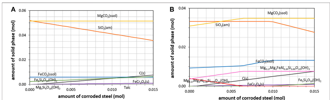
FIGURE 9 | Predicted effect of the corrosion of stainless steel grinding beads on carbonation products ( T = 175^\circ\text{C} , P_{\text{CO}_2} = 20 bar) for slag described as (A) system 1 (major metal oxides only) and (B) system 2 (major and minor metal oxides).
