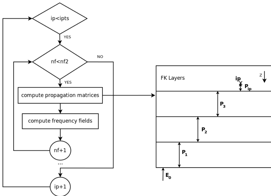
Figure A1. Original FK computation flowchart. A first loop is performed over the ipts nodes on the edges of the mesh inside which a second loop is performed over the nf2 frequencies.
