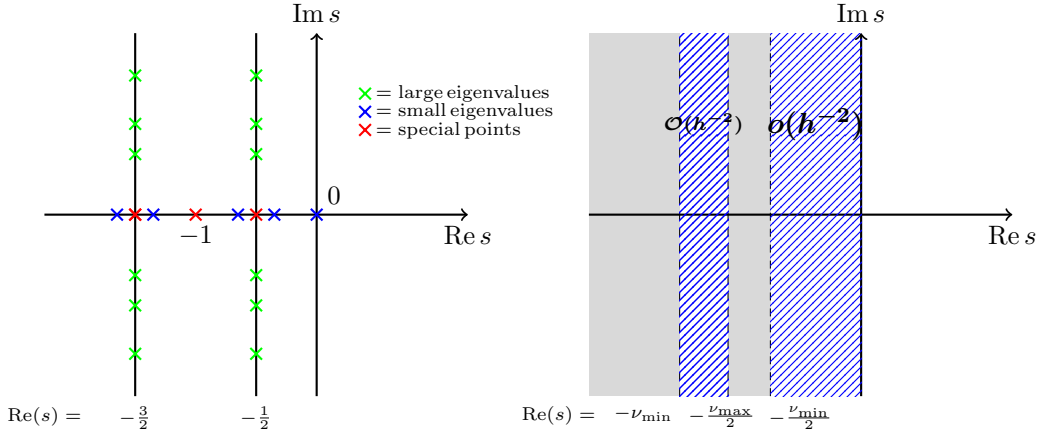
FIGURE 1. On the left: resonance spectrum of a closed hyperbolic surface \Sigma [DFG]; colouring describes the nature of the resonance. On the right: band structure of a contact Anosov flow on a 3-manifold given by Theorem 1. In dashed blue regions we have only finitely many resonances, with semiclassical resolvent bounds written using \mathcal{O} and o notation; gray regions are not covered by the theorem.
