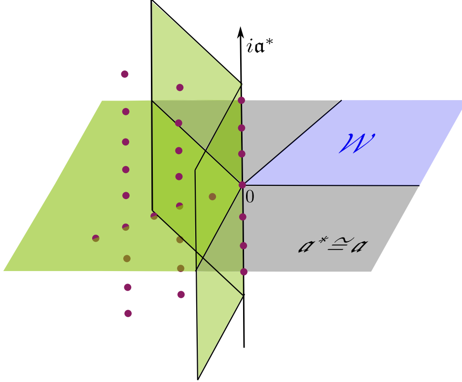
FIGURE 1. Schematic sketch of the location of the resonances in \mathfrak{a}_\mathbb{C}^* . Note that in order to draw the at least 4 dimensional space \mathfrak{a}_\mathbb{C}^* the imaginary direction ia^* has been reduced in the drawing to a one dimensional line. The blue cone depicts the positive Weyl chamber \mathcal{W} and the green region illustrates the region (1.3) in which the resonances can occur. The leading resonances discussed in Theorem 3 are located at the tip of this region.
