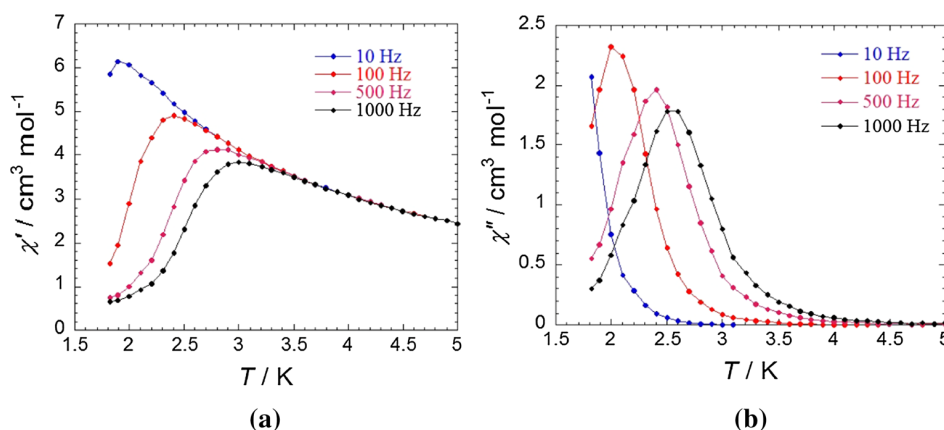
Fig. 7 Ac susceptibility of complex 1 -0.5C 6 H 14 in a 3.5 G field oscillating at 10, 100, 500, and 1000 Hz: in-phase signal ( \chi' ) and out-of-phase signal ( \chi'' ) versus T
