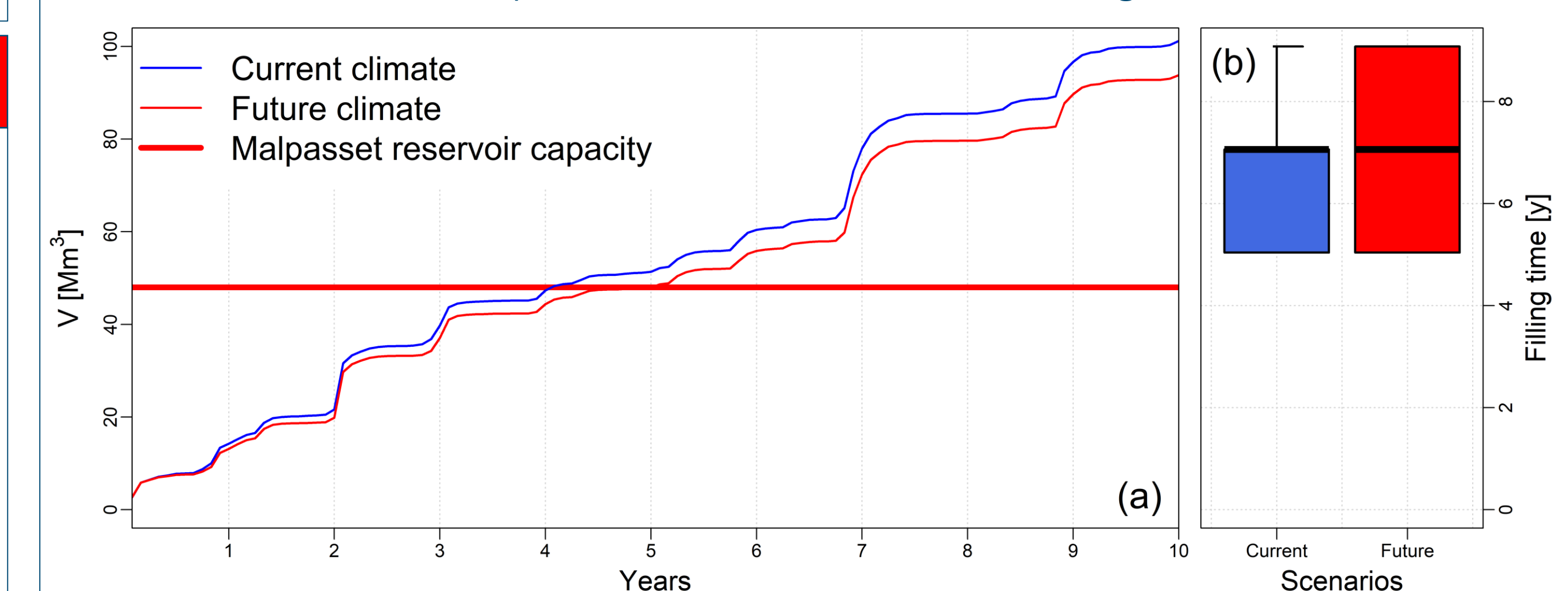
Fig. 6 a: Comparison of the water volumes in the reservoir for the current and future climate, b: Distribution of the filling times simulated from the GR2M simulated flows.
