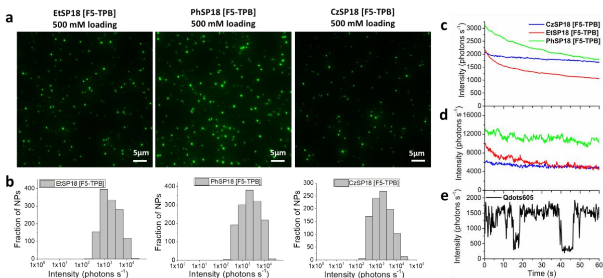
Figure 7. Single-particle characterization of polymeric NPs loaded with 500 mM EtSP18/[F5-TPB] , PhSP18/[F5-TPB] and CzSP18/[F5-TPB] . a. Single-particle fluorescence images of dye-loaded NPs. b. Corresponding distribution histograms of NPs brightness. c. Photobleaching profiles of polymeric NPs loaded with 500 mM CzSP18 , EtSP18 and PhSP18 dyes with [F5-TPB] counterion. d. Single-particle traces of the NPs. e. Single-particle trace of Qdots 605.
