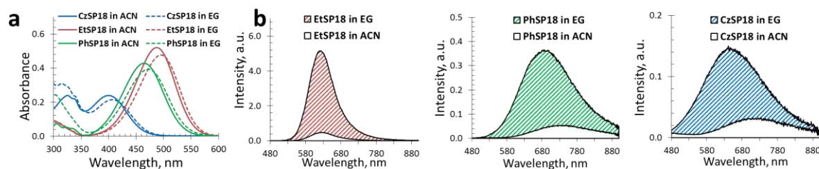
Figure 2. Spectroscopic studies of new dyes iodides in organic solvents of different viscosity. Absorption (a) and fluorescence (b) spectra of EtSP18 , PhSP18 and CzSP18 in acetonitrile and ethylene glycol ( \lambda_{\text{exc}} = 400 \pm 2 nm for CzSP18 and 460 \pm 2 nm for PhSP18 and EtSP18 ). In the fluorescence spectra, the curves were divided by absorbance values at the excitation wavelength. Concentration of dyes was 10 and 1 \mu\text{M} for absorption and fluorescence spectroscopy, respectively.
