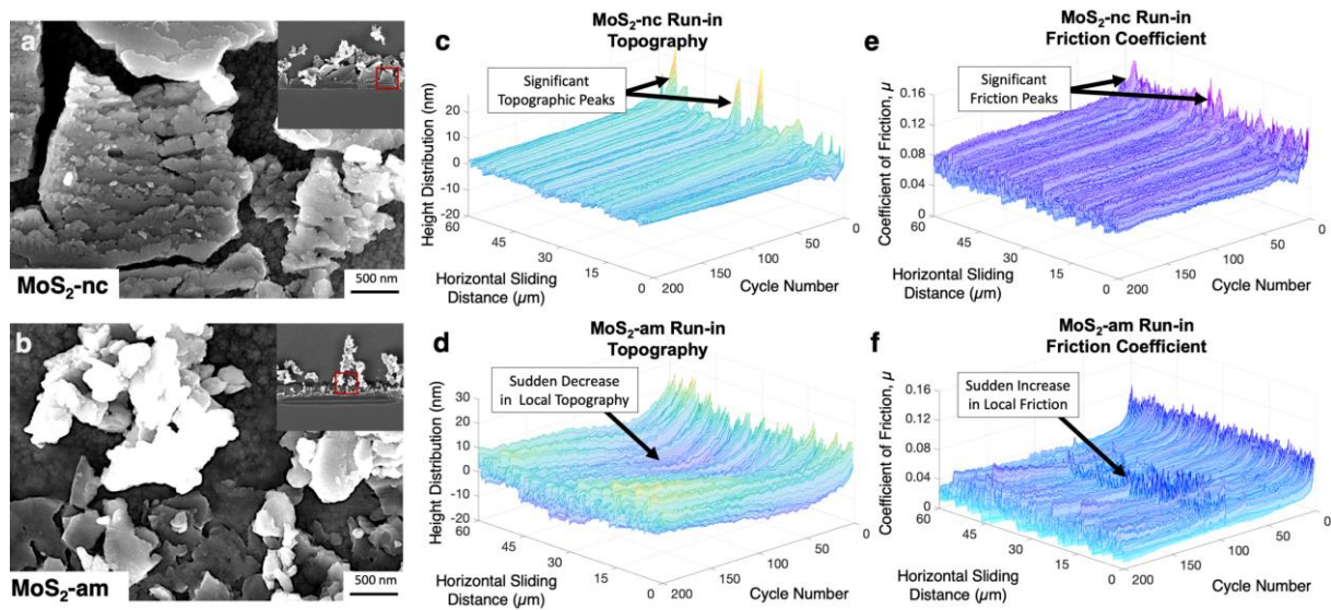
Figure 4. Run-in wear, topographic, and frictional characteristics; Wear debris following 150 cycles at the edge of the wear track for a) MoS 2 -nc, b) MoS 2 -am; 3D mapping of run-in friction and topographic characteristics of c) MoS 2 -nc topography, d) MoS 2 -am topography, e) MoS 2 -nc friction coefficient; f) MoS 2 -am friction coefficient
