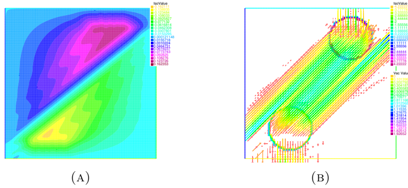
FIGURE 4. (A): the potential u , (B): the flow \phi .
