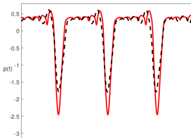
Figure 3: Two waveforms for the mouthpiece pressure calculated with the minimum model. The total length is the same for the two cases: L=1.3\text{m} . Solid line: x_1 = 0.2\text{m} . Dotted line: x_1 = 0.3\text{m} . The pressure p(t) is reduced by the static closure pressure.
