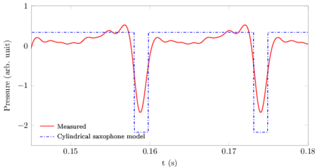
Figure 2. Periodic signal of the mouthpiece pressure of a barytone saxophone, and the approximation by a rectangle signal (pure Helmholtz motion). The duration of the of negative pressure state, which corresponds to the reed beating, is common to the different notes with different values of the equivalent length \ell of the truncated cone.
