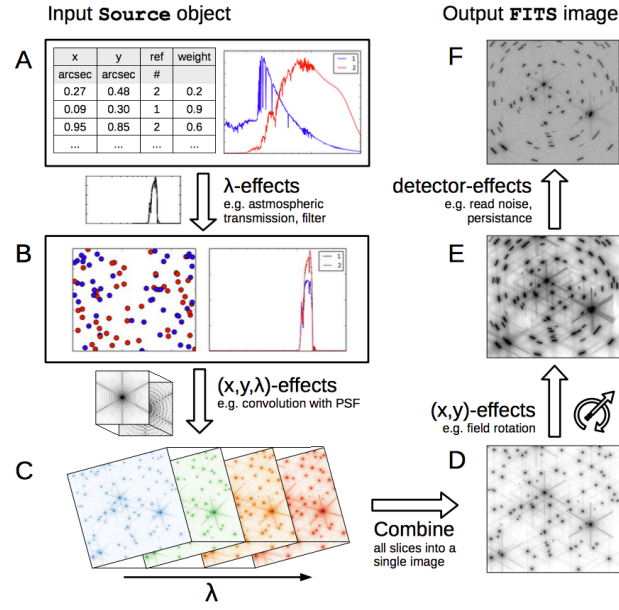
Fig. 3. SimCADO data model, representing the flow of events from the creation of the source object (here a mock open cluster) to the output FITS image. More details in Leschinski et al. (2016)
