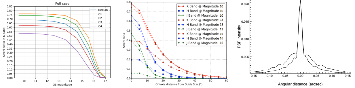
Fig. 1. Left: K-band SCAO performance vs. the guide star magnitude for the different ESO atmospheric conditions. Note that the complete SCAO performance is obtained from these end-to-end AO simulations results and additional instrumental error terms (130 nm rms left for these instrumental contributors to fulfil the SCAO performance specifications of SR=60%). Middle: Off-axis SCAO performance under Q2 seeing conditions for magnitudes R=10, 13 and 16. Right: SCAO PSF radial and transversal cuts obtained for L_0=25 m and 60 arcsec off-axis distance. The maximum intensity is equal to the K-band Strehl ratio, i.e. about 2%.
