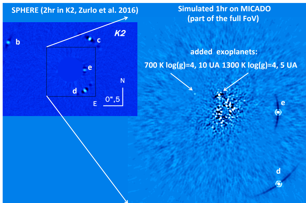
Fig. 2. Example of post ADI image showing: on the left : actual detection of 4 planets around HR 8799 by SPHERE (Zurlo et al. 2016) in K2 band ( \lambda = 2.255\mu\text{m} ), on the right : detection of simulated planets around HR 8799 using the actual measured flux for the closest planet d and e and using synthetic planet spectrum from EXOREM (Charnay et al. 2018) assuming 1 hour observation on MICADO at the same wavelength.
