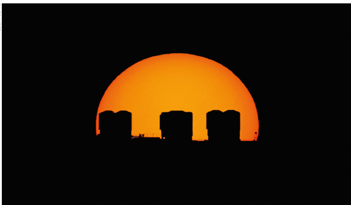
The 8.2-metre Unit Telescopes of the Paranal Observatory in silhouette against the Sun.
