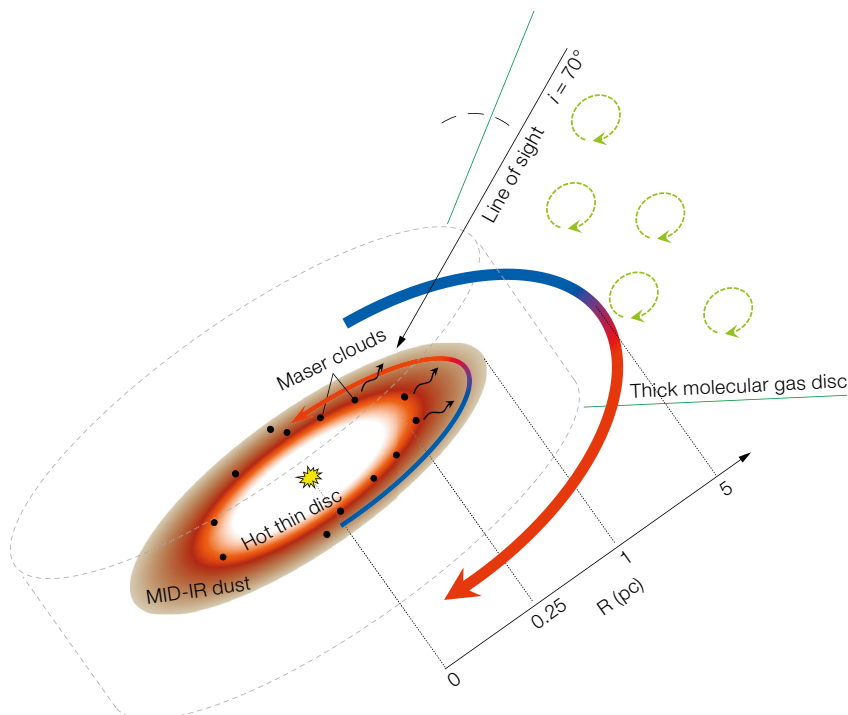
Figure 2. Sketch of the observed central structures. The K-band emission traces the inner rim of a thin disc of hot gas and dust, at or close to the dust sublimation radius of 0.24 pc. The inner water masers are cospatial with the hot K-band dust. The masers stretch out to 1 pc (Gallimore et al., 2001). Mid-infrared observations show warm dust on roughly the same scales as the outer masers, likely originating
