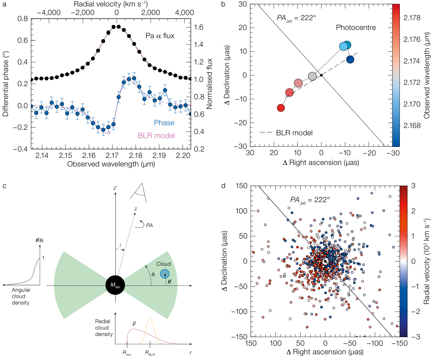
Figure 1. GRAVITY spatially resolves the broad emission line kinematics of 3C 273. (a) Paα line profile (black) and averaged differential phase (blue), showing non-zero phases and a change of sign across the broad emission line. (b) Photocentre positions measured at each line channel, showing a clear separation between red and blue which corresponds to a velocity gradient at a position angle perpendicular to the large-scale radio jet of 3C 273 (black line).
