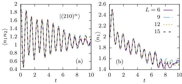
Fig. 4 Evolution of local observables for the Hamiltonian H_1 . a Correlations between adjacent sites \langle n_1 n_2(t) \rangle for different system sizes and the initial state |(210)^n . b Density on one site \langle n_1(t) \rangle .
