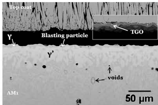
Fig. 6. End-of-life microstructure of the TBC-PA5 sample after 1170 cycles at 1100 °C (SEM-BSE).
