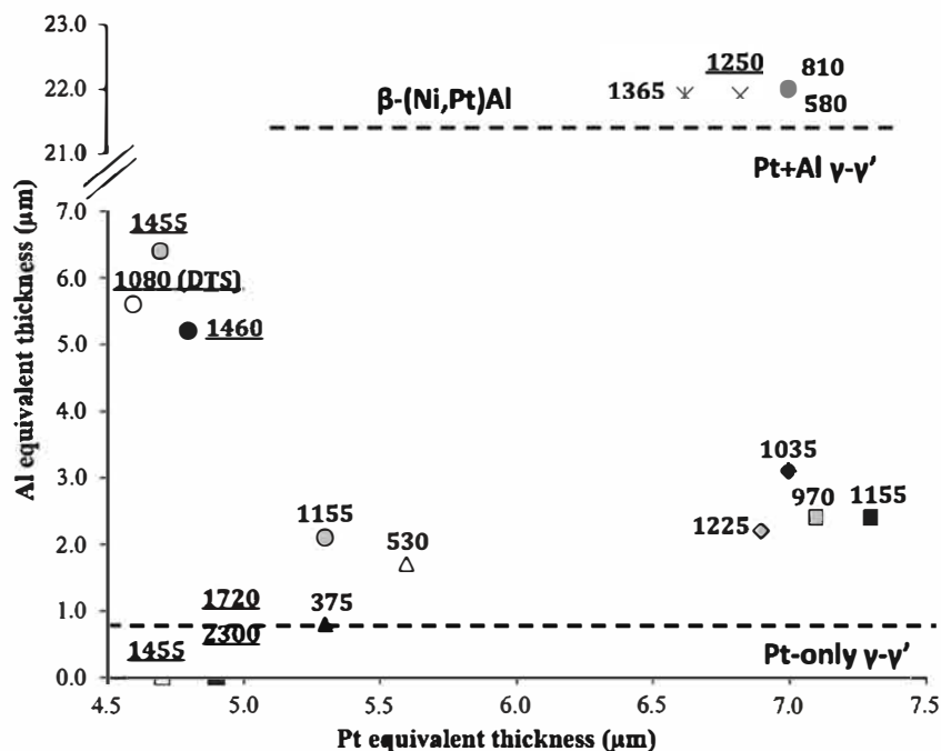
Fig. 7. Life span of all the systems depending on their Pt and Al initial additions (Pt and Al equivalent thicknesses). DTS = Desktop Spalling. Results from Run 2 are underlined.
