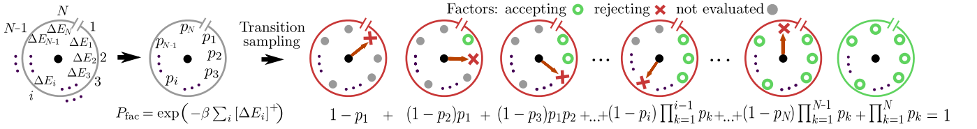
FIG. 1: Sketch of the clock sampling technique. The inhomogeneous Bernoulli process described by Eq. (2) can be decomposed into N+1 clocks, where the i th clock ( i \leq N ) alarms of the first occurrence of a rejection event at time i and the (N+1) th clock, with no alarm, represents an acceptance event. Such a process can be sampled within O(1) computational complexity.
