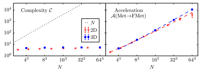
FIG. 4: Complexity \mathcal{C} (left) and acceleration \mathcal{A} (right) for the 2D ( \beta=1 , red circle) and 3D ( \beta=0.693 , blue square) RKKY Heisenberg spin systems, comparing the clock FMet method to the Metropolis algorithm. The dashed red and blue lines respectively represent fits to aN and aN/\log N + b .
