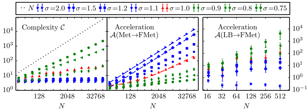
FIG. 3: Complexity \mathcal{C} (left) and acceleration \mathcal{A} for the clock FMet algorithm for the 1D ( \beta=1 ) long-range Ising spin glass, compared to the Metropolis algorithm (middle) and the LB algorithm (right). The dashed blue and red lines respectively represent fits to aN and aN/(\log N)^2 + b .
