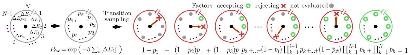
FIG. 1: Sketch of the clock sampling technique. The inhomogeneous Bernoulli process described by Eq. (2) can be decomposed into N+1 clocks , where the i th clock ( i \leq N ) alarms of the first occurrence of a rejection event at time i and the (N+1) th clock , with no alarm, represents an acceptance event. Such a process can be sampled within O(1) computational complexity.
