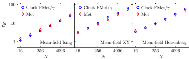
FIG. 2: Integrated autocorrelation time \tau_E of the energy for the ferromagnetic mean-field O(n) model expressed in units of system sweeps. The values for the clock FMet algorithm are normalized by \gamma (Eq. (8)).
