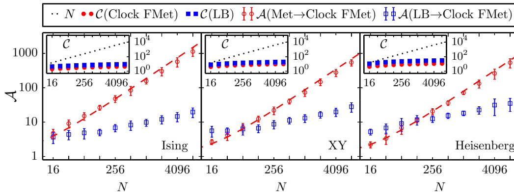
FIG. 5: Acceleration \mathcal{A} for the disordered mean-field O(n) model in random fields at \beta=n (complexity \mathcal{C} in insets). The clock FMet method exhibits important acceleration \mathcal{A} , compared to both the Metropolis (red circles) and the LB cluster algorithm (blue squares). The dashed red line represents a fit to aN + b .
