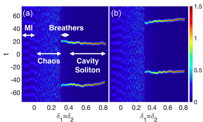
FIG. 3. Stationary state power distributions Y_{SS} in fiber 1 (a) and Z_{SS} in fiber 2 (b) over time which emerge in a Möbius resonator composed of two identical fibers, as a function of common detuning from the pump \delta_1 = \delta_2 . The steady states are obtained by sequentially incrementing both \delta_1 and \delta_2 in steps of 0.01, then propagating for 500 round trips of the dual Ikeda map Eq. (1). Parameters: A_{in} = 0.166 , \beta_{3,n} = 0 , \eta_1 = \eta_2 = -1 , \theta = 2/15 , and \alpha_i = 1/100 . Different regimes of dynamic steady-state behavior are indicated with white labels and arrows; the steady state is time-independent for detunings outside these ranges.
