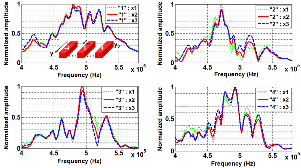
Fig. 16 Displacement amplitude measured along the width of the elements (points x_1 , x_2 , x_3 ) at the frequency 481 kHz
