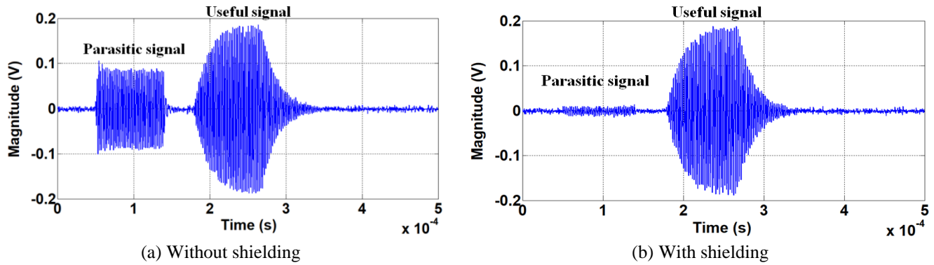
Fig. 11 Signal measured using a PVDF hydrophone
