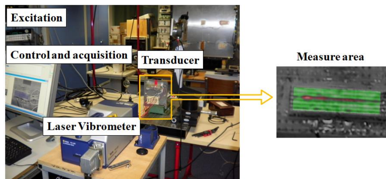
Fig. 4 Displacement measurement set-up
