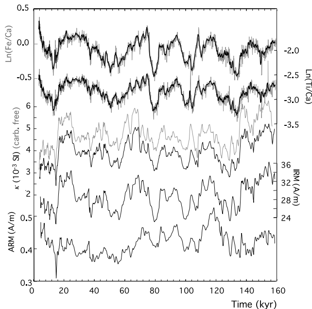
Figure 6. Ti/Ca and Fe/Ca log ratio (and a 7-points running average) and bulk magnetic parameter ( \kappa , IRM and ARM) curves versus time in core MD06-3067. The magnetic susceptibility calculated on a carbonate-free basis is also reported on the same vertical scale as \kappa by the gray curve.
