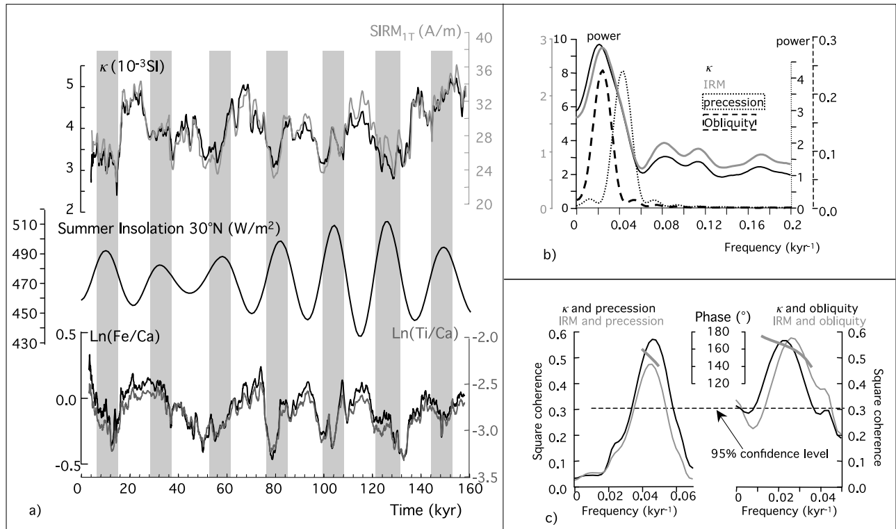
Figure 9. Relationship between magnetic concentration in core MD06-3067 and insolation. (a) Comparison between IRM, \kappa , Ln(Fe/Ca) , Ln(Ti/Ca) (both reported as 7-points running average curves), and the summer (1 June to 31 August) mean insolation curve calculated at 30^{\circ}N using Laskar et al. [2004] solution; (b) Blackman-Tukey spectrum analysis calculated using Analyseries software [Paillard et al., 1996] for \kappa (black), IRM (gray), and the insolation shown in Figure 9a after filtering at 23 kyr (named “precession,” dotted line) and 40 kyr (named “obliquity,” dashed line); (c) squared coherence between \kappa (black), IRM (gray), and the 23 kyr-filtered insolation curve on the left and between \kappa , IRM, 40 kyr-filtered periodicity on the right. The phases between the magnetic parameters and the insolation ones are reported in degrees for the time domain in which the curves are significantly correlated.
