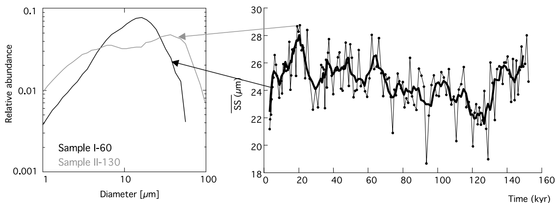
Figure 8. Inorganic mean grain size in core MD06-3067. (right) Sortable silt mean size (thin black curve) and running average curve (thick line) versus time. (left) Examples of two spectra obtained for fine (black curve) and coarse (gray curve).
