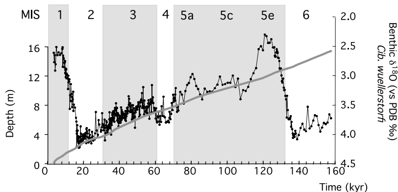
Figure 2. Benthic oxygen isotope record and age–depth relationship (gray line) in core MD06-3067. MIS stands for marine isotopic stages.
