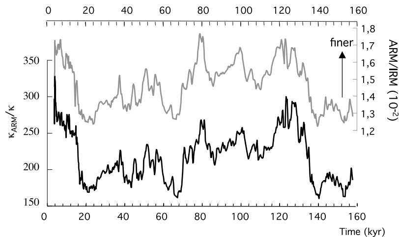
Figure 4. Magnetic grain size in core MD06-3067 expressed by the ratios ARM/IRM (in gray) and \kappa_{ARM}/\kappa (in black). Both show the same variations versus time.
