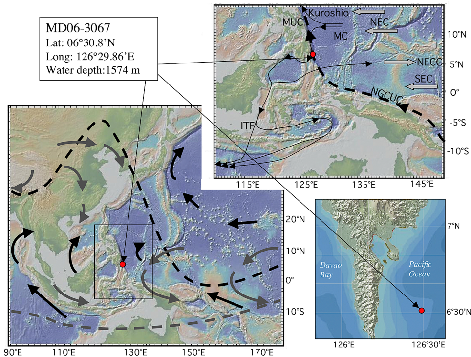
Figure 1. Maps showing the location of core MD06-3067. (left) Summer (dashed black line) and winter (dashed gray line) positions of the ITCZ and associated directions of trade winds. (top right) Main oceanic water masses (MC, Mindanao Current; MUC, Mindanao Undercurrent; NGCUC, New Guinea Coastal Undercurrent; ITF, Indonesian Throughflow; NEC, North Equatorial Current; NECC, North Equatorial Counter Current; SEC, South Equatorial Current). (bottom right) More precise location of the core with respect to the southern tip of Mindanao and the Davao Bay. The maps are constructed using GeoMapApp software.
