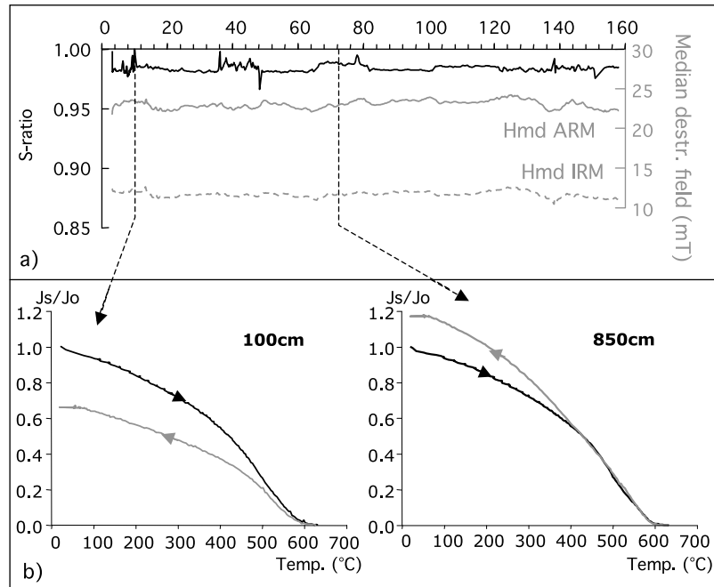
Figure 3. Magnetic parameters defining the magnetic mineralogy in core MD06-3067. (a) S\text{-ratio}_{-0.3T} (black line) and median destructive fields of ARM and IRM ( Hmd_{IRM} in dashed gray line and Hmd_{ARM} in continuous gray line); (b) two representative thermomagnetic curves obtained from different horizons with the heating curve in black and the cooling curve in gray. All indicate that the main carrier is low Ti content magnetite.
