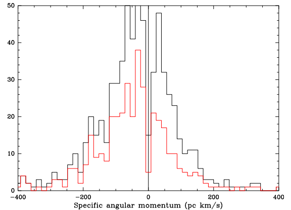
Fig. 4. Histogram of angular momenta for M 51 clouds. In black for the subsample S/N \geq 7 and in red for the subsample S/N \geq 10 . Note that the gradients in the higher S/N subsample are better defined (more prograde and with a more significant gradient). We have included a correction for beam-smearing as in B18. The angular momenta of the M 51 clouds are substantially higher than in M 33 (see middle panel of next figure).
