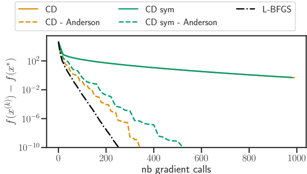
Figure 4: \ell_2 -regularised logistic regression, real-sim . Suboptimality as a function of the number of gradient calls on the 2000 first features of the real-sim dataset, Tikhonov strength set so that \kappa = 10^5 .
