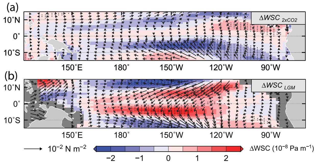
Figure 8. Wind changes in response to 2\times\text{CO}_2 and LGM forcing. Multimodel mean change in surface wind stress (arrows) and curl (WSC, colors) simulated by six coupled general circulation models (GCMs) in response to (a) doubling of atmospheric \text{CO}_2 ( 2\times\text{CO}_2 ) and (b) LGM forcing. Stippling is as in Figure 1.
