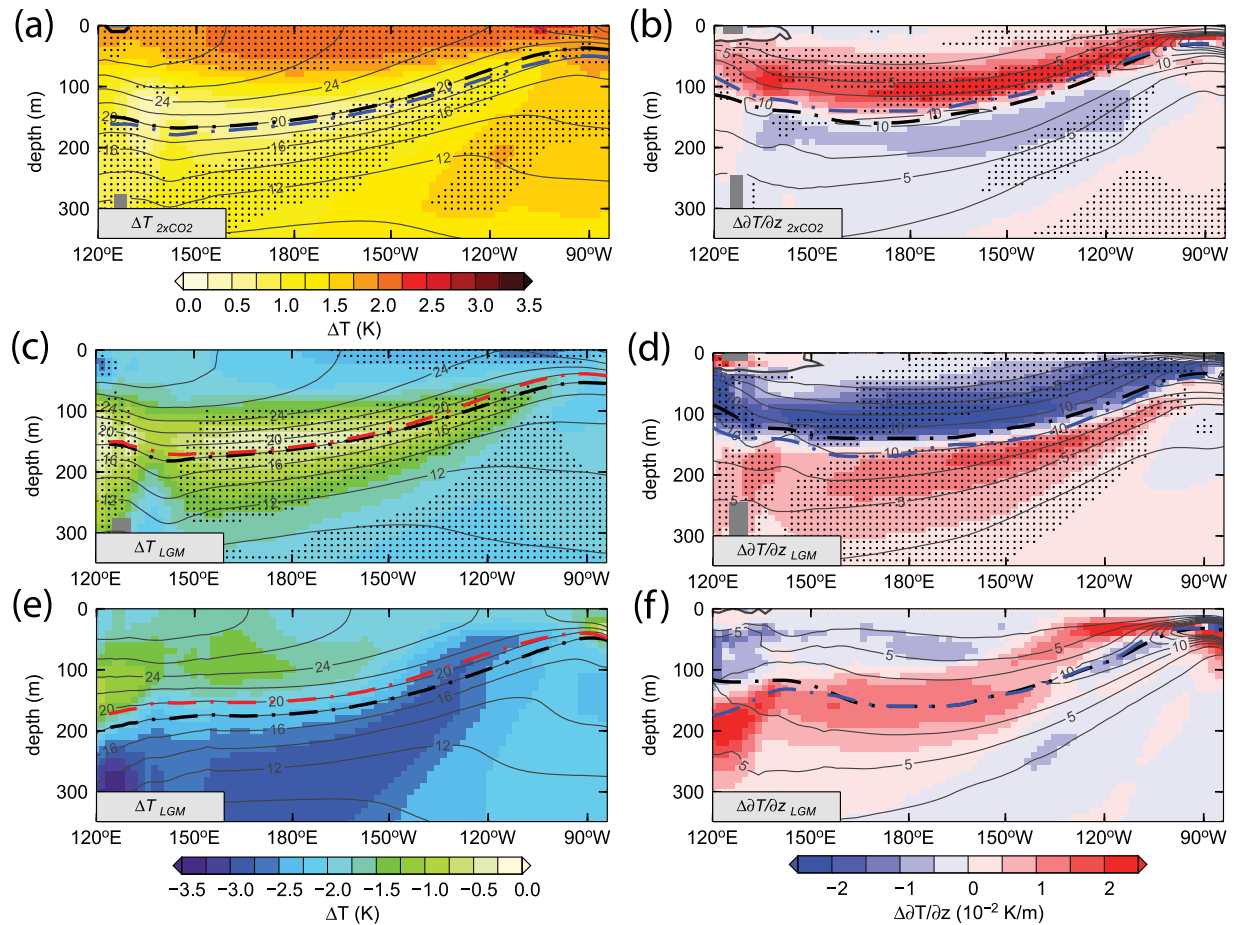
Figure 10. Response of the equatorial thermocline to 2\times\text{CO}_2 and LGM forcing. Multimodel change in equatorial Pacific Ocean (a) temperature and (b) vertical temperature gradient ( \partial T/\partial z ) simulated by six coupled GCMs in response to 2\times\text{CO}_2 forcing. Multimodel change in equatorial Pacific ocean (Figures 10c and 10e) temperature and (Figures 10d and 10f) \partial T/\partial z simulated by (Figures 10c and 10d) MIROC3.2, FGOALS-g1.0, and IPSL-CM4 (three-model ensemble mean) and by (Figures 10e and 10f) CCSM3.0 in response to LGM forcing. These four models simulate a stronger Walker circulation in response to LGM forcing. The changes in CCSM3.0 are shown separately because this model's subsurface response is substantially different than that of the remaining three models with a stronger Walker circulation. Stippling is as in Figure 1. In Figures 10a, 10c, and 10e the dash-dotted lines indicate the 20^\circ\text{C} ( 2\times\text{CO}_2 ) and 18^\circ\text{C} (LGM) isotherms in the control (black) and forced (red) experiments. In Figures 10b, 10d, and 10f the dash-dotted lines indicate the depth of the thermocline, i.e., the maximum of \partial T/\partial z , in the control (black) and forced (blue) experiments. The equatorial sections are averaged over the 2^\circ\text{S} and 2^\circ\text{N} latitude band. Contours show multimodel annual mean temperature and \partial T/\partial z simulated in the control experiment. \text{CI} = 2 \text{ K} (temperature) and \text{CI} = 2.5 \cdot 10^{-2} \text{ K m}^{-1} ( \partial T/\partial z ).
