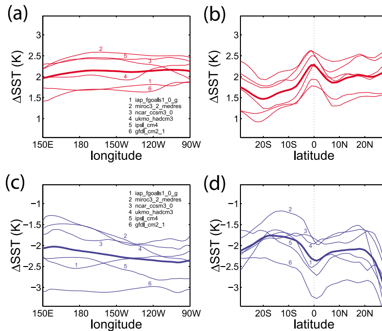
Figure 9. Signature of tropical Pacific warming and cooling. Change in surface temperature in the equatorial Pacific in response to (a) 2\times\text{CO}_2 (red) and (c) LGM forcing (blue) simulated by six coupled GCMs (thin lines) and their multimodel mean (solid line). The equatorial changes (Figures 9a and 9c) are averaged over 5^\circ\text{S} and 5^\circ\text{N} . Zonal mean change in surface temperature in the tropical Pacific in response to (b) \text{CO}_2 doubling and (d) LGM forcing simulated by six models (thin lines) and multimodel mean (solid line). The zonal mean changes (Figures 9b and 9d) are averaged from 150^\circ\text{E} to 90^\circ\text{W} .
