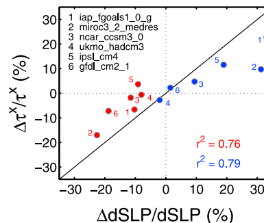
Figure 7. Changes in SLP gradient and zonal trade winds in the equatorial Pacific in response to 2xCO 2 and LGM forcing. Fractional change in zonal wind stress averaged over the equatorial Pacific (2°S–2°N) versus changes in sea level pressure gradient, as diagnosed by the east-west SLP difference (SLP), simulated by each model in response to 2xCO 2 (red) and LGM (blue) forcing.
