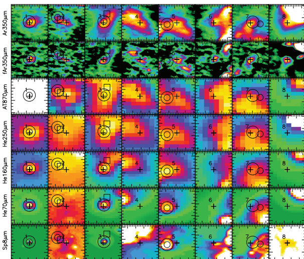
Figure C26. Same as Fig. C1 but for the SDC343 field.
