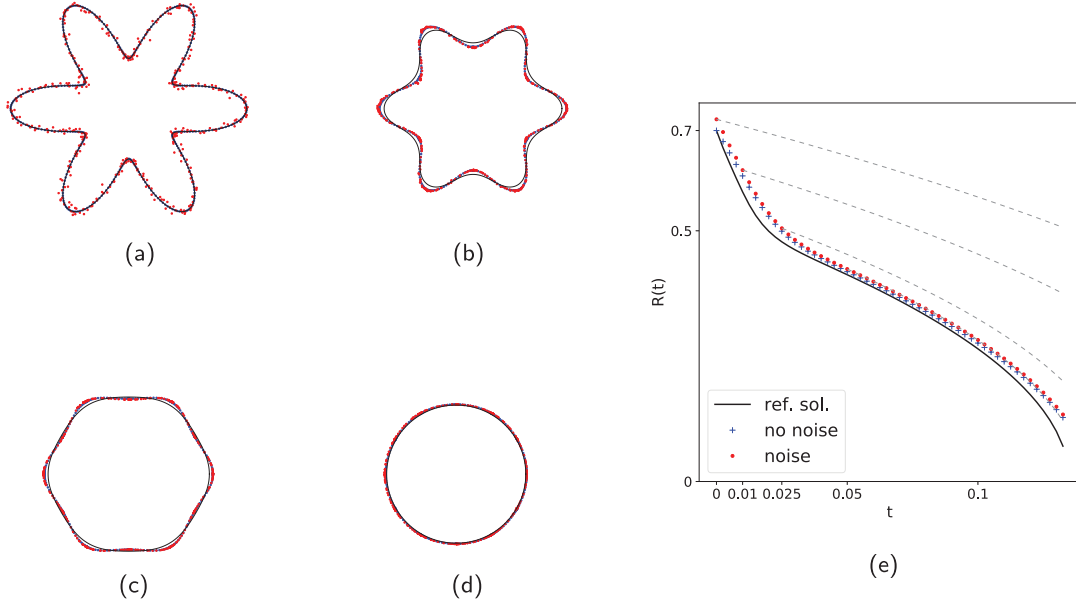
FIGURE 5. Left figure (a) to (d): Blue and red point clouds are the results given by our scheme without adding noise for the blue point cloud and with white noise of standard deviation 5/N for the red point cloud. The black curve is the reference solution. Right figure (e): we compute and represent the minimal radius R(t) of the circle (centered at 0) and including the points at time t , keeping the same parameters and color code as in the left figure. We moreover add grey dashed lines corresponding to the graph of t \mapsto \sqrt{R(t_0) - 2(t - t_0)} for t_0 \in \{0, 0.01, 0.025, 0.05\} and R(t_0) is the radius obtained for the initially noisy shape (red dots). (a) time t = 0 . (b) time t = 0.01 . (c) time t = 0.025 (d) time t = 0.05 .
