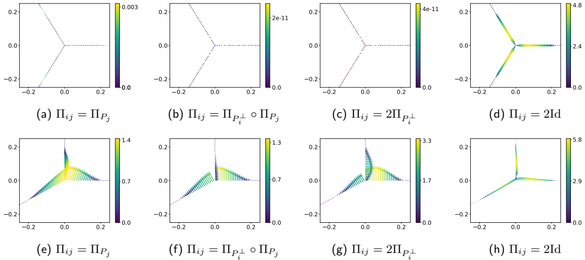
Figure 5. Computed mean curvature vector at junction point depending on the chosen projection operator.
