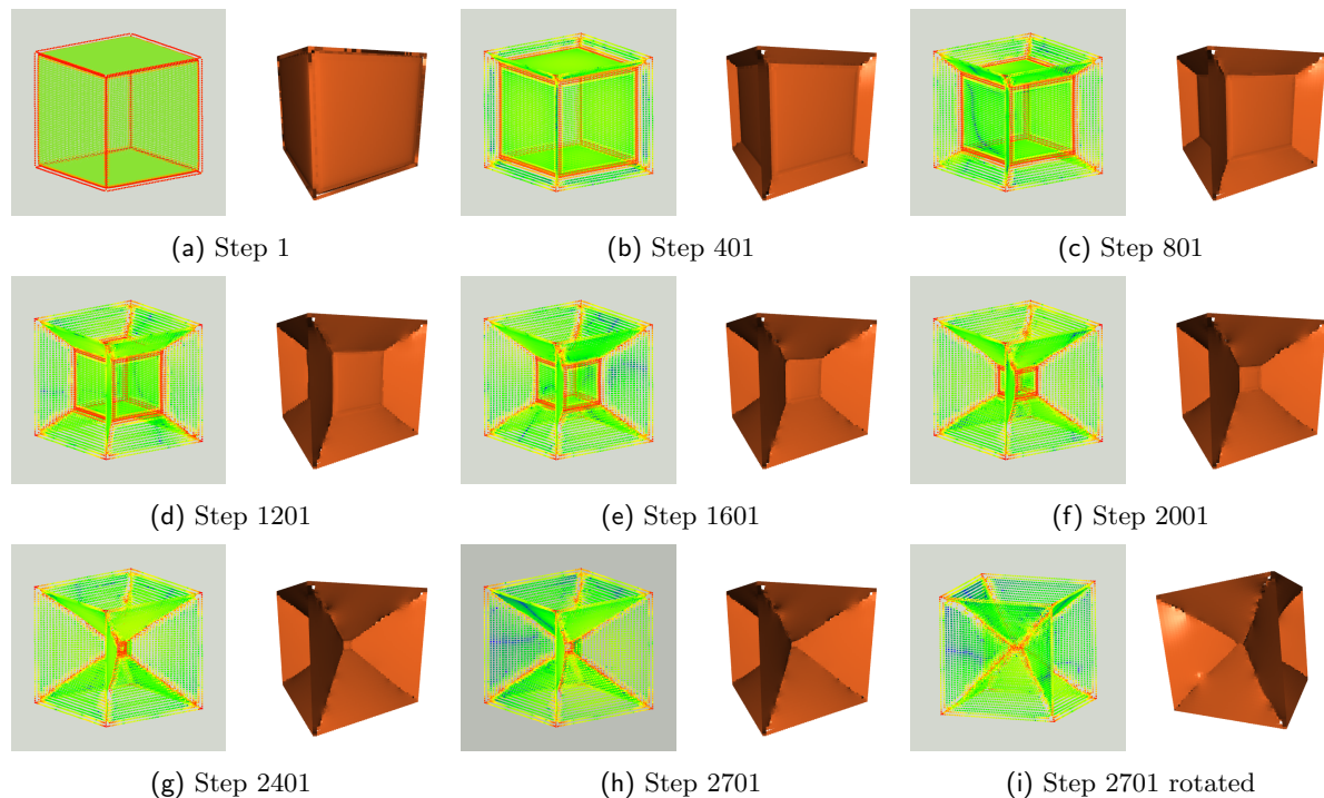
Figure 10. Different steps of the semi-linear scheme (47) performed on (the surface of) a cube whose edges are fixed, discretized with N = 18600 points and for a time-step \tau = 0.01 . Again, the norm of the approximate mean curvature vector is color coded on the left and on the right a shaded visualization of the point clouds using square shaped splats with proper point normals is shown.
