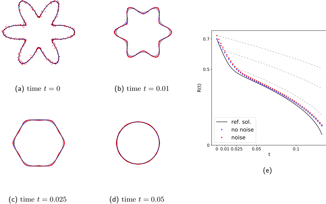
Figure 4. Left figure (a) to (d) : Blue and red point clouds are the results given by our scheme without adding noise for the blue point cloud and with white noise of standard deviation 5/N for the red point cloud. The black curve is the reference solution. Right figure (e) : we compute and represent the minimal radius R(t) of the circle (centered at 0) and including the points at time t , keeping the same parameters and color code as in the left figure. We moreover add grey dashed lines corresponding to the graph of t \mapsto \sqrt{R(t_0) - 2(t - t_0)} for t_0 \in \{0, 0.01, 0.025, 0.05\} and R(t_0) is the radius obtained for the initially noisy shape ( red dots).
