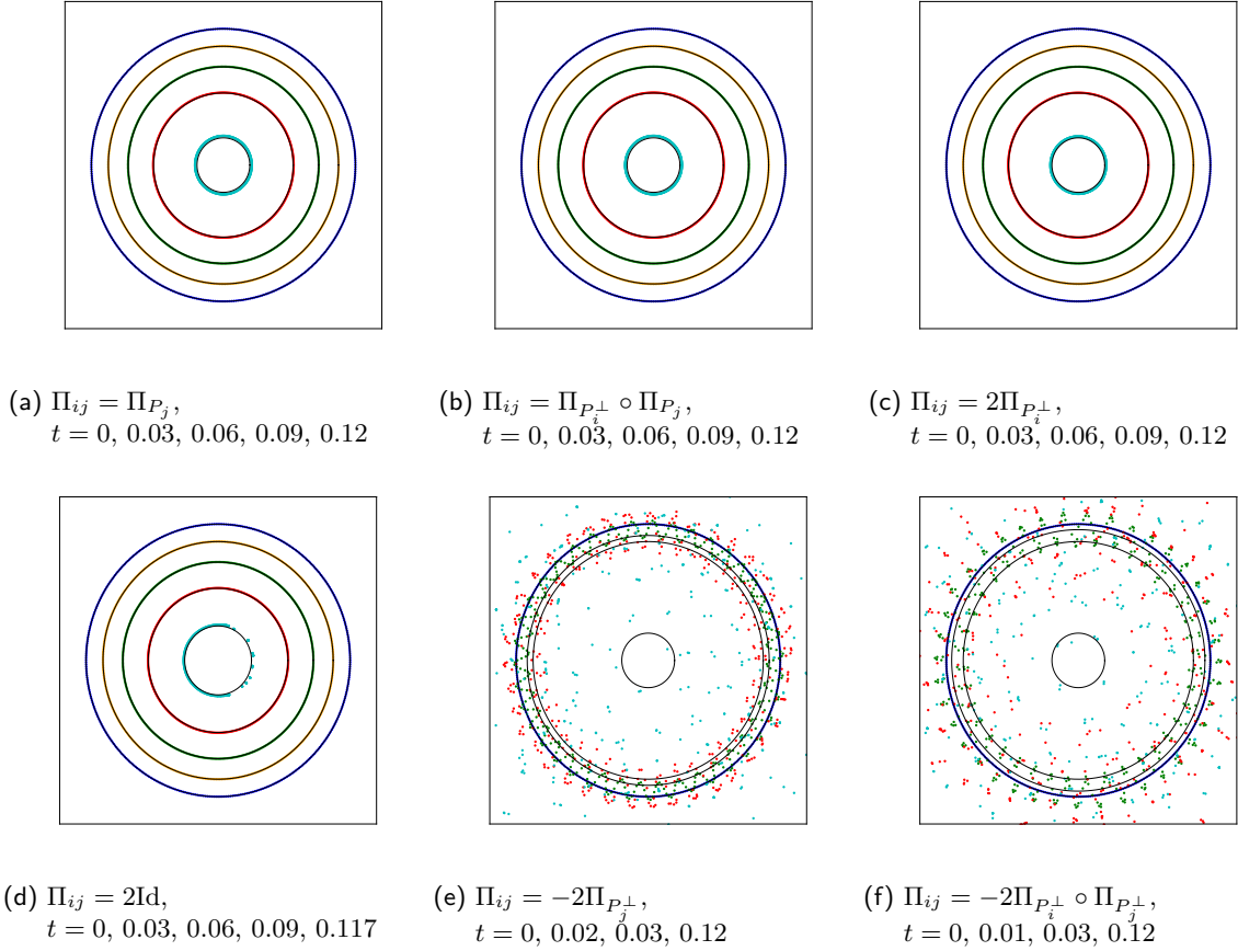
Figure 1. Comparison of the results given by the semi-implicit scheme (47) for different choices of operator \Pi_{ij} . The test is performed on a circle uniformly discretized with N = 400 points, the number of points for computing the mass is fixed to k_\delta = 3 , the number of points for the regression is fixed to k_\sigma = 17 and the number of points for the computation of curvature is fixed to k_\varepsilon = 15 , the time step is \tau = 0.1/N = 0.0005 . The numerical solutions and the exact solutions in black are represented at same times t . Simulations are stopped then resulting in clutter due to noise amplification.
