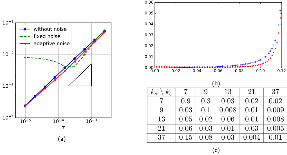
Figure 3. (a) Decay of the mean error (49) at time T = 0.1 when the time step \tau \in \{2^{-k}/N : k = 0, \dots, 8\} is refined, N = 400 . Black triangle indicates slope 1 in log–log scale. (b) Error e(t) represented with respect to time t , for \tau = 6.25 \cdot 10^{-4} , in red with initial white noise (of standard deviation 1.25 \cdot 10^{-3} ) and in blue without noise. (c) Error e(0.1) for different numbers of points k_\sigma used for computing tangent and k_\varepsilon used for computing curvature.
