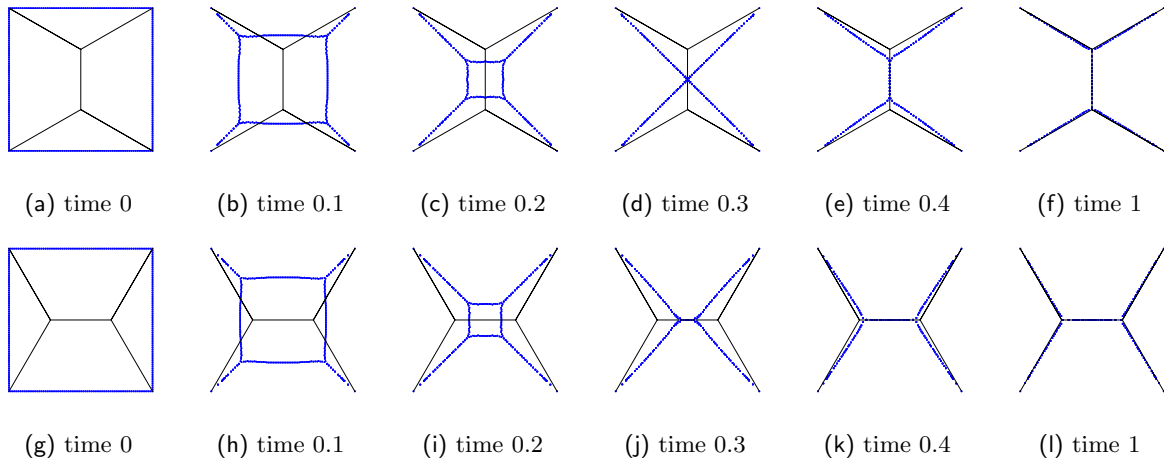
Figure 8. Evolution of a square whose corners are fixed to one (a)–(f) or the other (g)–(l) Steiner tree connecting the 4 fixed corners.
