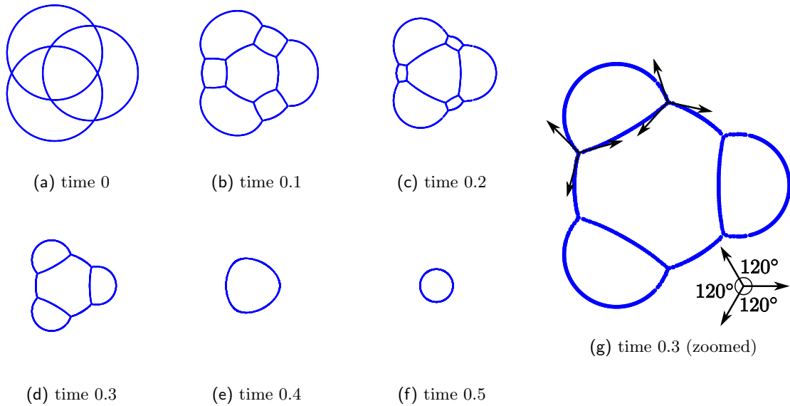
Figure 7. Evolution of three circles towards one circle under discrete curvature flow.
