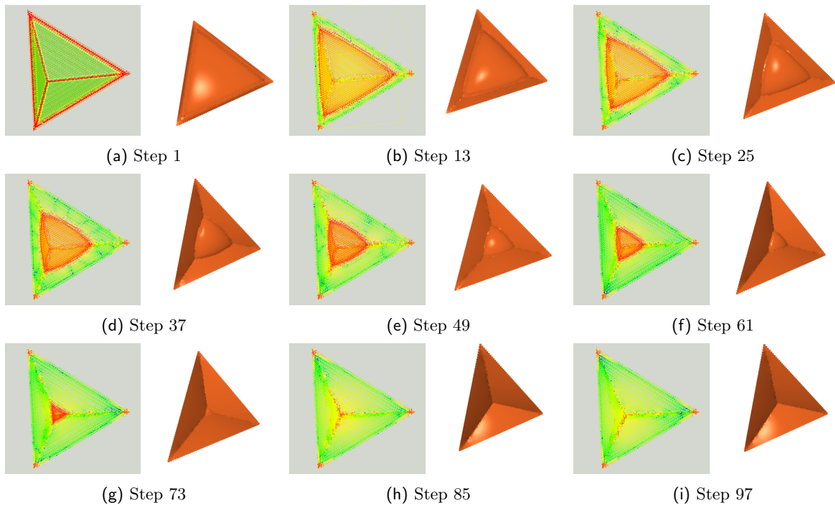
Figure 9. Different steps of the semi-linear scheme (47) performed on (the surface of) a tetrahedron whose edges are fixed, discretized with N = 6052 points and for a time–step \tau = 0.005 . The norm of the approximate mean curvature vector is color coded on the left and on the right a shaded visualization of the point clouds using square shaped splats with proper point normals is shown.
