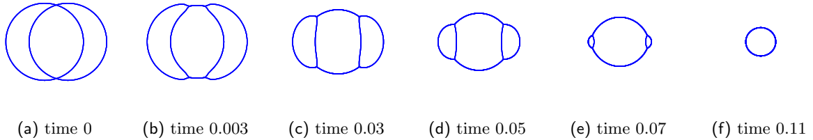
Figure 6. Evolution of two crossing circles under discrete curvature flow.
