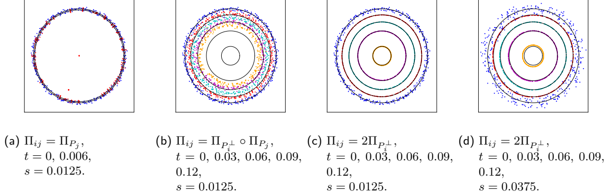
Figure 2. Comparison of the results given by the semi-implicit scheme (47) for different choices of operator \Pi_{ij} when adding white noise. The test is performed on circle uniformly discretized with N = 400 points, the number of points for computing the mass is fixed to k_\delta = 3 , the number of points for the regression is fixed to k_\sigma = 17 and the number of points for the computation of curvature is fixed to k_\varepsilon = 15 , the time step is \tau = 0.1/N = 0.0005 . The numerical solutions and the exact (black line) solutions are represented at same times t . To the initial circle is added a Gaussian noise with standard deviation s = 5/N = 0.0125 in 2a–2c and s = 15/N = 0.0375 in 2d.
