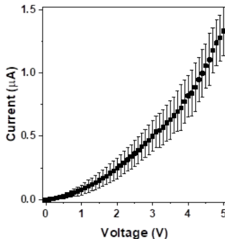
Figure 2. Averaged I-V characteristics of twelve as-prepared ITO/100 nm [Fe(HB(tz) 3 ) 2 ]/Al junctions recorded in ambient conditions at rates of \pm 100 mV/s.
