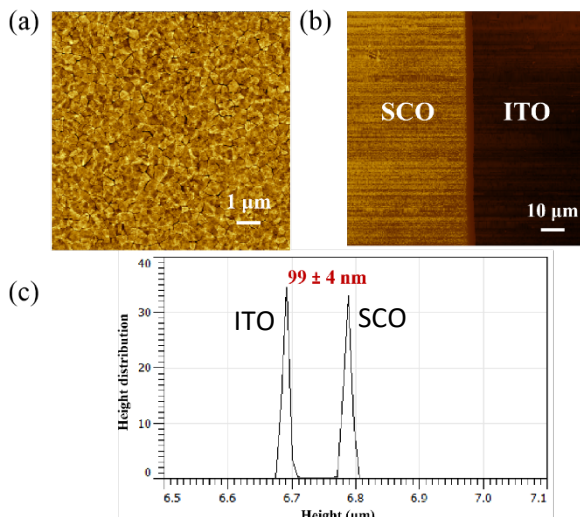
Figure 1. a) 10 \times 10 μm AFM topography image of a [Fe(HB(tz) 3 ) 2 ] thin film. b) 100 \times 100 μm AFM topography image of a [Fe(HB(tz) 3 ) 2 ] thin film and the bare ITO substrate and c) the corresponding height distribution histogram.
