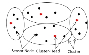
Fig. 2. Clustering Concept.
