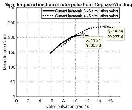
Fig. 10: Mean torque curves for the proposed 15-phase machine
