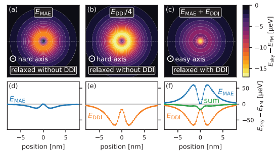
Figure 2. Energy density distribution with respect to the FM state at B = 750 mT. (a) and (b): The skyrmion was relaxed with an easy axis in-plane anisotropy of 13 \mu\text{eV} and without DDI: (a) MAE contribution and (b) DDI contribution. (c) skyrmion relaxed with both DDI and an easy axis anisotropy out-of-plane of 60 \mu\text{eV} . (d), (e) and (f): radial energy density distribution showing the MAE (d), the DDI (e) and both contribution (f). The integral of (a) and (c) are of comparable magnitude with 13.8 meV and 11.8 meV, respectively.
