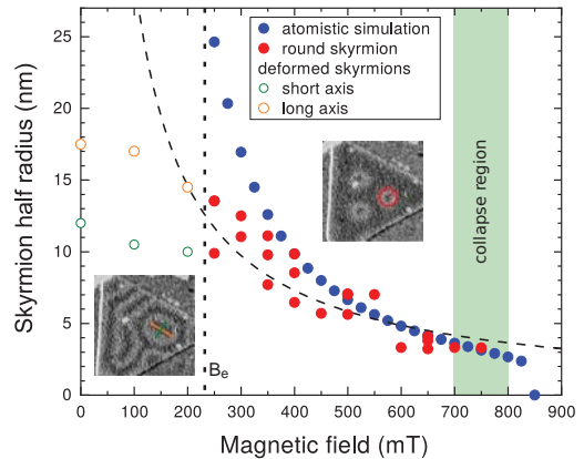
Figure 1. Theoretical (blue filled circles) values of \sigma/2 of the skyrmion versus applied magnetic field in Co/Ru(0001) together with the experimental values for round skyrmions B > B_e \approx 230 mT as illustrated in the right inset. At B < B_e , the skyrmions are elongated and both the radii along the long (orange) and short (green) axis are plotted as illustrated in the left inset. The black dashed curve is a fit to a/B . At fields in the shaded green area, annihilation of skyrmions was experimentally observed. The insets are differential conductance maps of the TAMR signal of 130 \times 130 nm, V = -350 mV, I = 2 nA, modulation: U = 60 mV. left inset: B = 0 mT, right inset: B = 400 mT.
