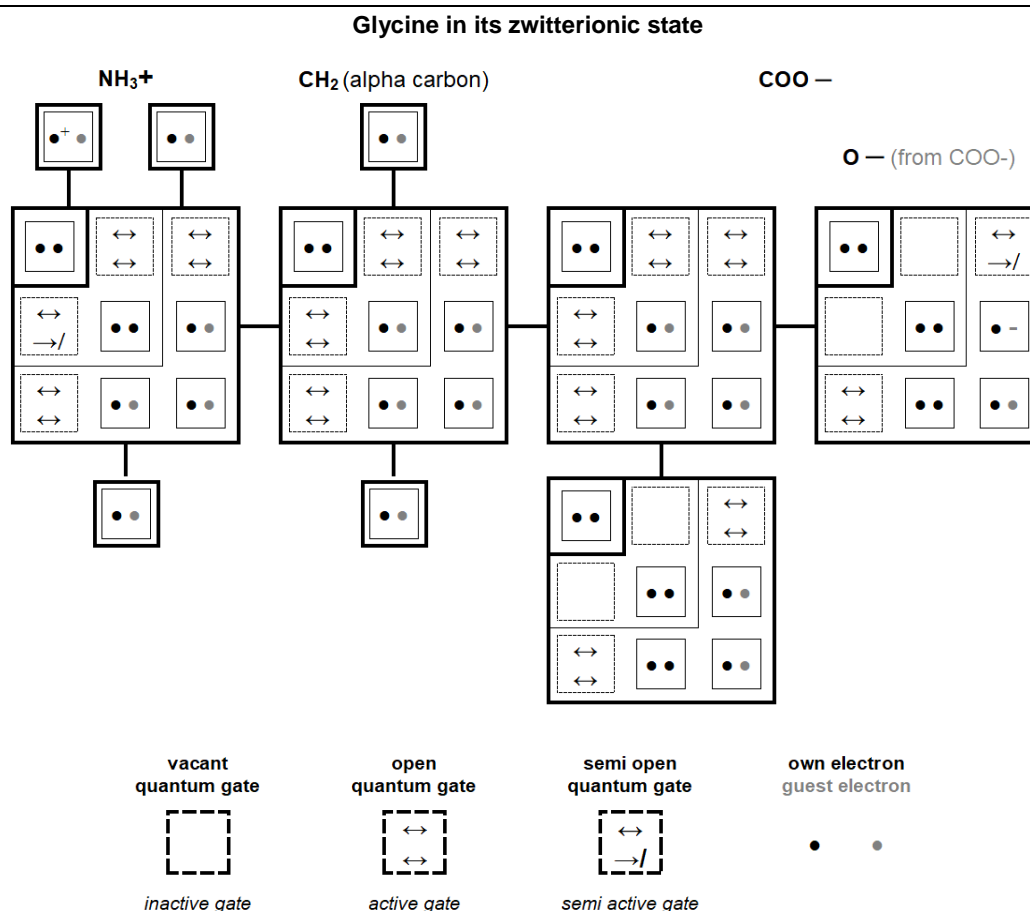
Fig. 12 Graphical quantum representation of chemical groups \text{NH}_3^+ , \text{CH}_2 (alpha carbon) and \text{O}^- (from \text{COO}^- ) of amino acid Glycine in its zwitterionic state. Own electrons (●) and guest electrons (◐). See Fig. 10 also.
