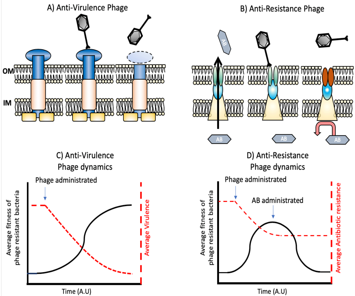
Figure 1. Phage steering of bacterial virulence and antibiotic resistance. Selection for bacterial resistance to phages at specific targets reduces bacterial virulence (A and C) or antibiotic resistance (B and D). As seen in C, the fitness of resistant bacteria (black line) increases due to phage pressure, while virulence (red line) declines. D shows a similar interaction, but this time focusing on antibiotic resistant mechanisms. The fitness of phage-resistant bacteria (black line) increases as phage replicate, and there is coetaneous decline in average antibiotic resistance (red line). Subsequent administration of antibiotics would reduce the fitness of these now antibiotic sensitive cells.
