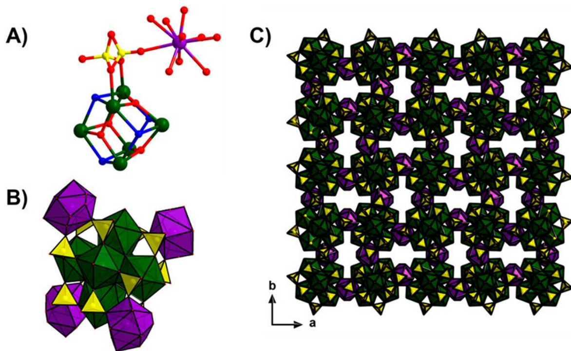
Figure 2. Representations of U-U_6 . (A) Ball-and-stick representation of the connectivity between the hexamer and monomer units via a disordered sulfate. For the U_6O_4(OH)_4 unit, U^{IV} are green spheres, O^{2-} are red spheres, and OH^- are blue spheres. The monomer U^{IV} is purple, and S (disordered over two half-occupied sites) of bridging SO_4^{2-} are yellow spheres. (B) Illustration of the tetrahedral arrangement of the monomers around the U_6 unit. Purple polyhedra are the U^{IV} monomers, green polyhedra are the U^{IV} of the hexamer, and yellow polyhedra are sulfates. (C) Framework view down the c axis. The color scheme is the same as that in part B.
