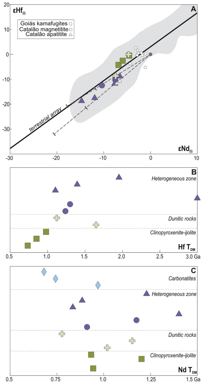
Fig. 5. (A) Initial \epsilon\text{Hf} vs. Initial \epsilon\text{Nd} diagram for analyzed Jacupiranga samples. Initial \epsilon\text{Nd} values from Chmyz et al. (2017), Goiás kamafugites (Carlson et al., 2007) and Catalão rocks (Guarino et al., 2017) are shown for comparison. Grey field represents oceanic and crustal data used to define the terrestrial array of Vervoort et al. (1999). Dashed vectors are models from Nowell et al. (2004) and show the isotopic evolution of MARID metasomites from an initial BSE composition over 1–1.5 Ga. (B) Distribution of \text{Hf } T_{\text{DM}} and (C) \text{Nd } T_{\text{DM}} model ages for analyzed Jacupiranga samples. Symbols are as in Fig. 4.
