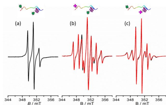
Fig 3. RT EPR spectra of equimolar mixtures of (a) mixture 1: N_{TAIL} S407C P and P_{XD} K496C P , (b) mixture 2: N_{TAIL} S407C PP and P_{XD} K496C P , (c) mixture 3: N_{TAIL} S407C P and P_{XD} K496C PP . The spectra shown in panels (b) and (c) have been simulated using the ROKI
