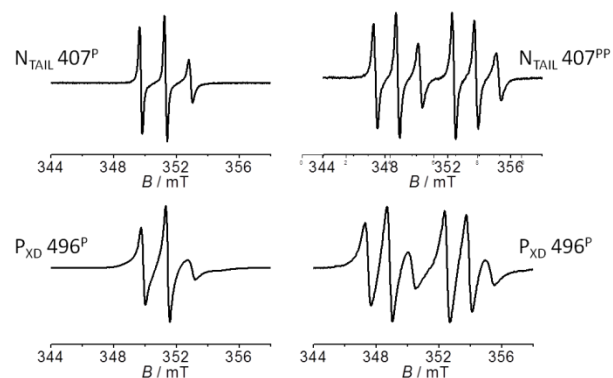
Fig. 2 Amplitude normalized RT EPR spectra of N_{TAIL} S407C P/PP (upper line) and P_{XD} K496C P/PP (lower line). Main recording parameters: microwave power 10mW, magnetic field modulation amplitude 0.1mT.
