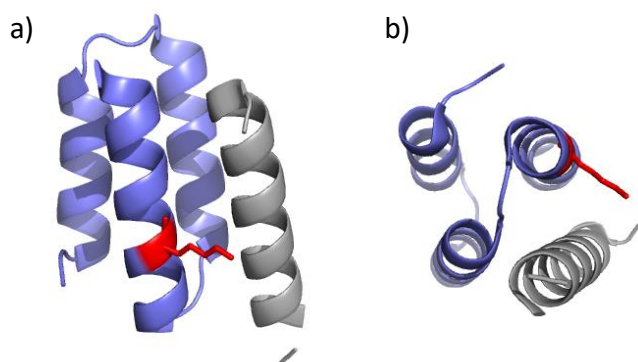
Fig. 1 Crystal structure of the MeV chimera between P_{XD} (residues 459–507) and the N_{TAIL} region encompassing residues 486–504 (pdb code 1T60 32 ). Lysine 496 of P_{XD} is highlighted in red. (a) lateral view and (b) bottom view.
