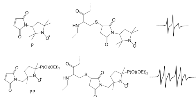
Scheme 1 Chemical structures of nitroxide radicals: 3-maleimido-2,2,5,5-tetramethyl-1-pyrrolidinyloxy (P) and {2-[(diethoxyphosphoryl)-5-[(2,5-dioxo-2,5-dihydro-1H-pyrrol-1-yl)methyl]-2,5-dimethylpyrrolidin-1-yl] oxidanyl (PP) and their link to cysteine residues with an illustration of the typical 3- or 6-line EPR signatures.
