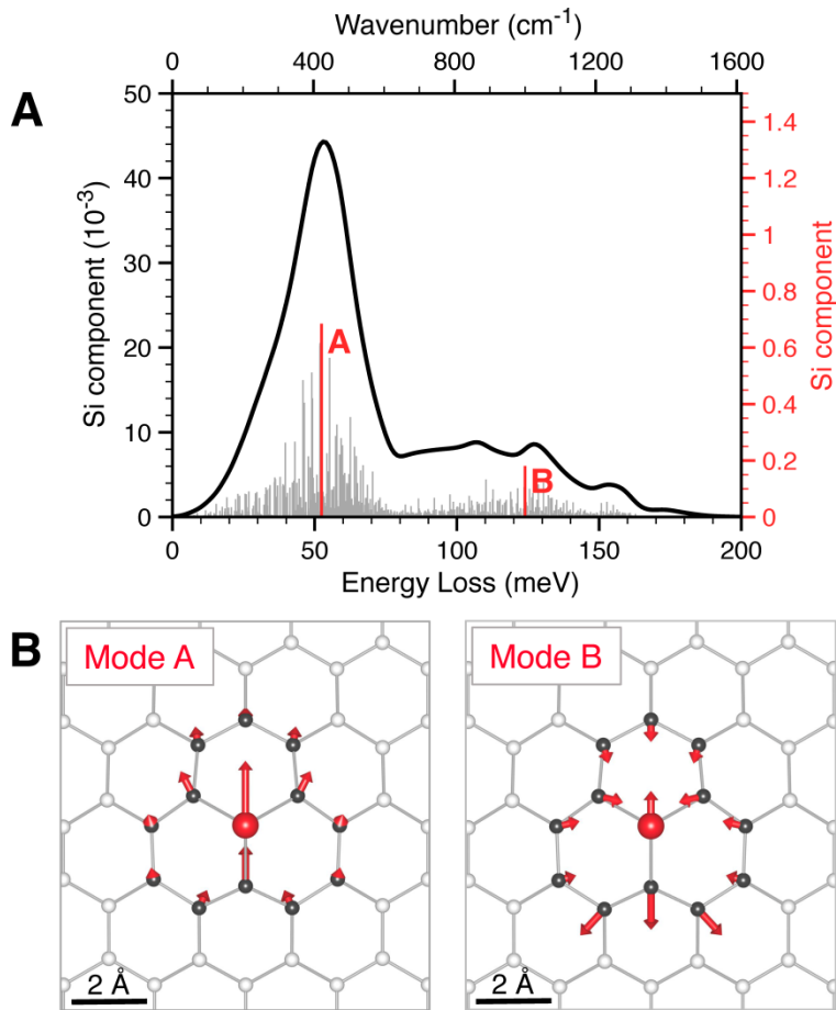
Fig. 3. Localized components of the Si vibrations. (A) Gray bar-histogram: square of the phonon eigenmodes of the 96×96 supercell projected on the in-plane Si atom component. Black line: in-plane component of the phonon DOS projected on the Si atom (same as the "Si" PPDOS in fig. 2) obtained by broadening the gray bar-histogram with a 2.0 meV FWHM Lorentzian. The red bar-histogram is calculated from a 13-atom fragment centered on the impurity. Two dominant modes, denoted A and B, are observed. (B) Atomic model of the 13-atom fragment (the Si atom is in red), with relative atomic displacements for modes A and B indicated as arrows whose length is proportional to the displacement amplitude.
